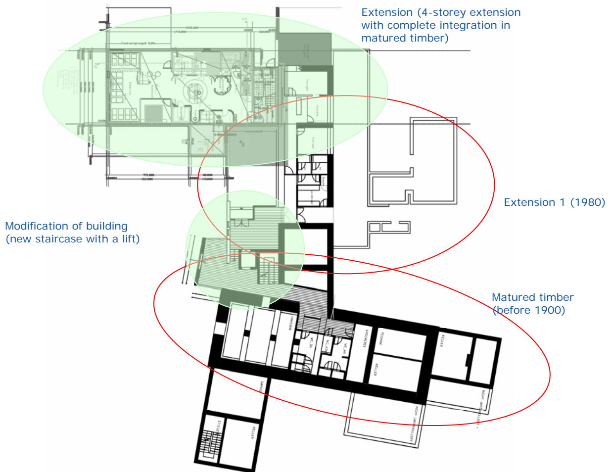
Plan view of the whole complex of buildings with the different construction stages
