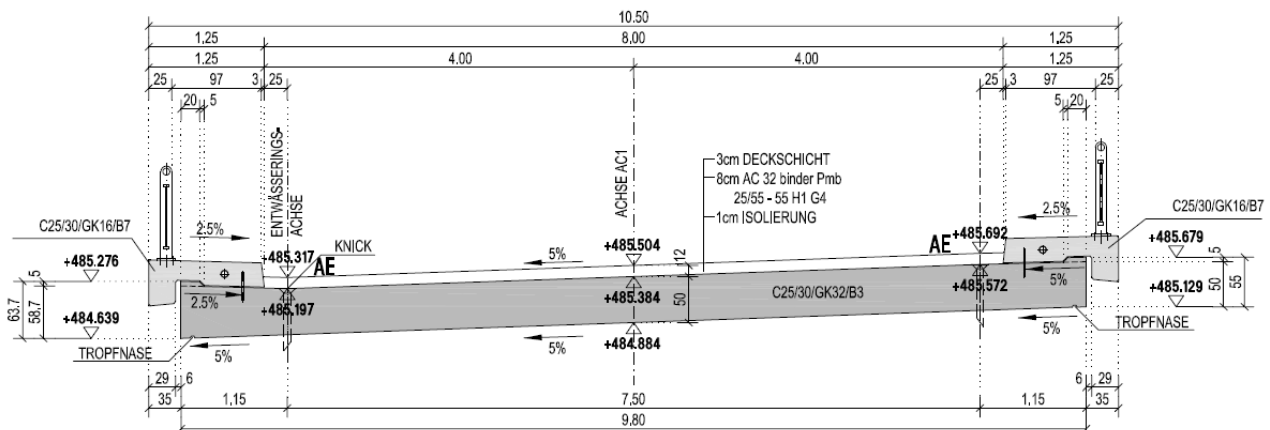
Typical cross-section
