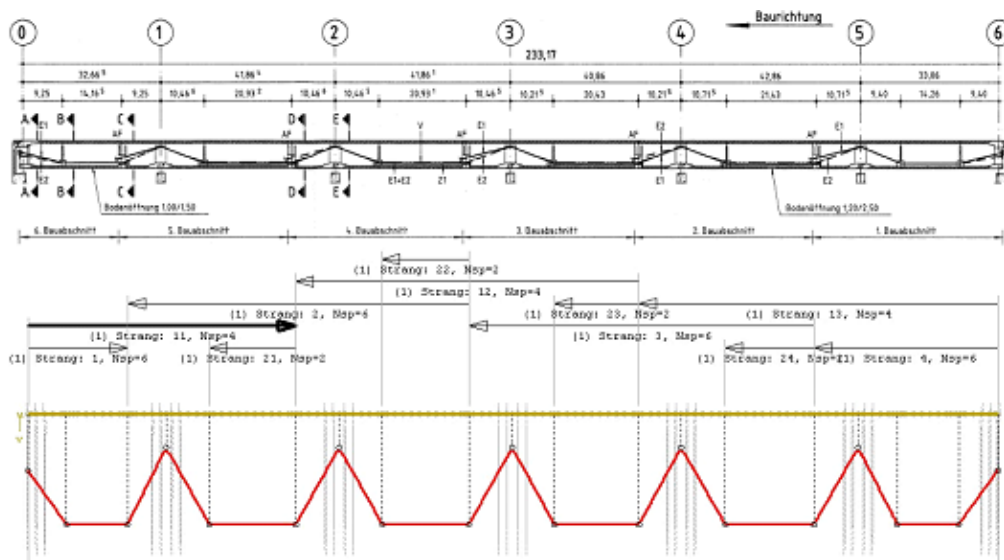
External pre-stressing
