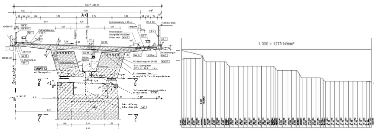
Cross-section with pre-stressing deviator
